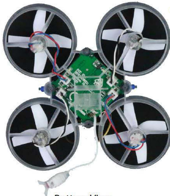
Bottom View Motor Connections
